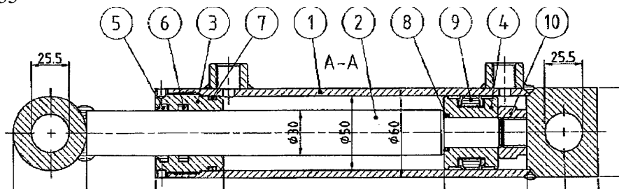
Cylinder 50/30-150
