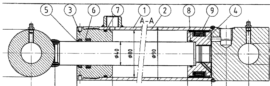
Cylinder 80/40-350 (91805)
